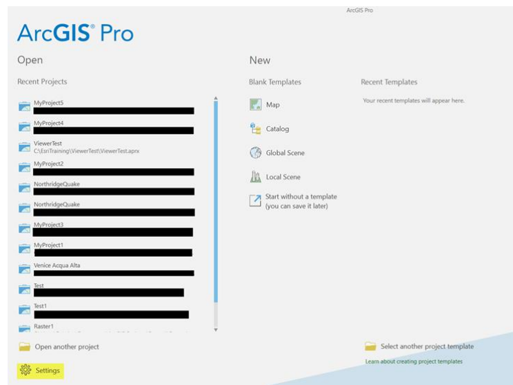
Gambar 1. Tab settings
