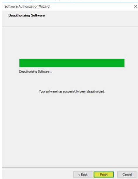
Gambar 7. Proses selesai
