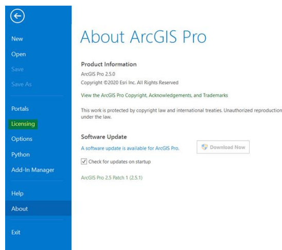
Gambar 2. Tab licensing
